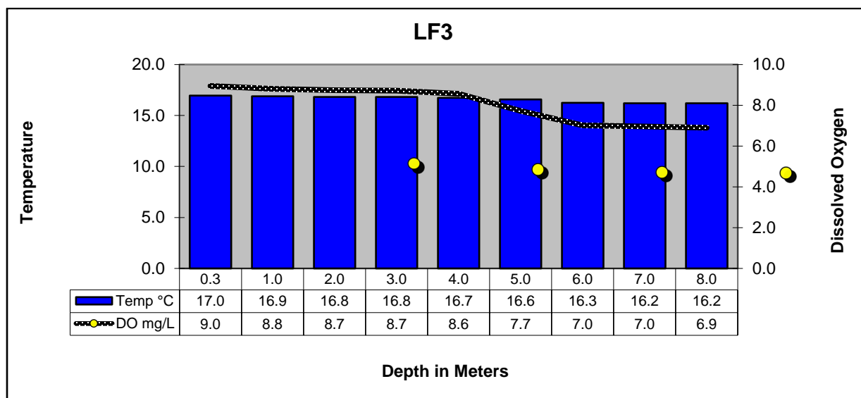
LAKE FORK RESERVOIR MID-ARM IN CANEY CREEK ARM AT FM515
